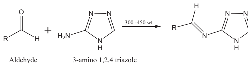
Scheme 1. Synthesis of Schiff's base from 3-amino-1,2,4-triazole and different aldehydes.
