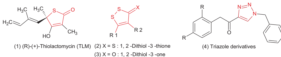
Fig. (1). Chemical structure of thiolactomycin, 1, 2-dithiol-3-thione (2) and (3) 1, 2-dithiol-3-one.
