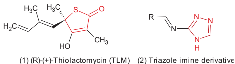
Fig. (2). Chemical structure of TLM and triazole imine.
