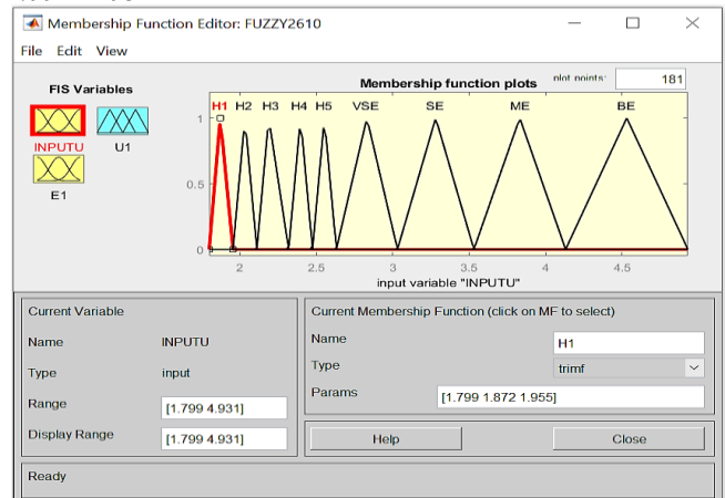
Fig. 9: Membership functions of first input variable of FLC.
