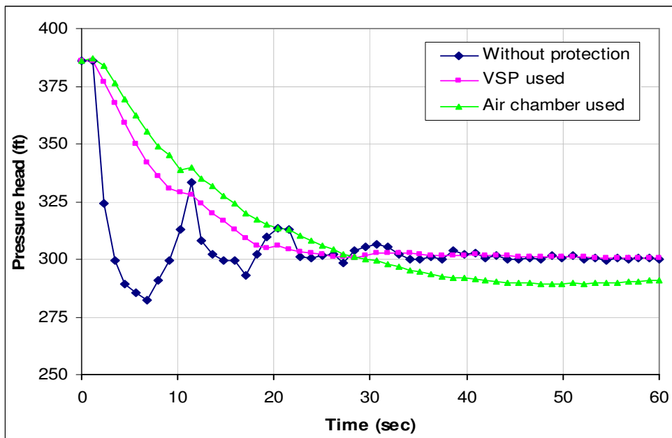
Figure 10: Effect of protection device on the local transient pressure at downstream end of pipe 6.
