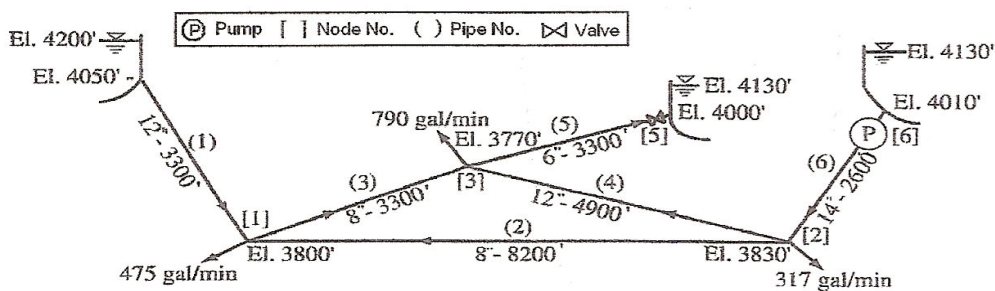
Figure 1: Case study network layout
