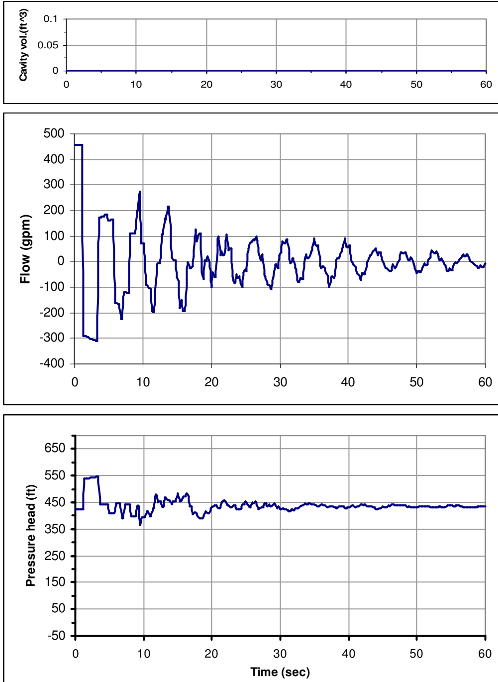
Figure 3: Transient history (Pressure, Flow & cavity volume) at the upstream end of Pipe 5 (junction 3), using closing rate (I).
