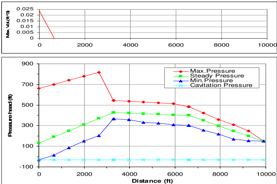
Figure 5: Pressure and cavity volume along path (TCV-1 → J-3 → J-1 → R-1), due to valve closing rate (I)
