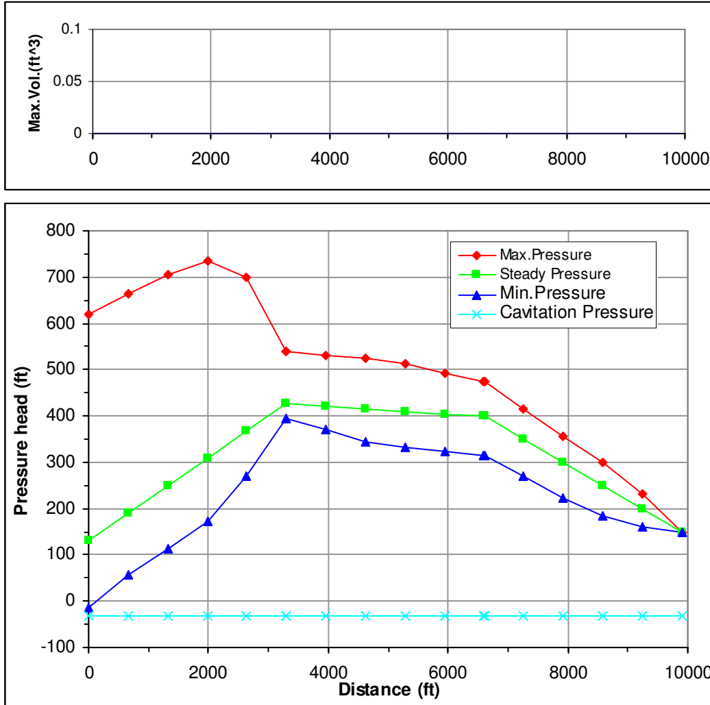
Figure 6: Pressure and cavity volume along path (TCV-1 → J-3 → J-1 → R-1), due to valve closing rate (III).
