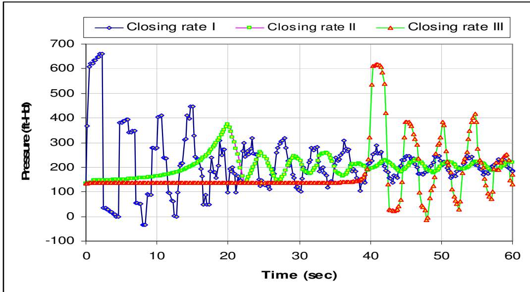
Figure 4: Effect of valve closing rate on local transient pressure head at the upstream end of the gate valve.
