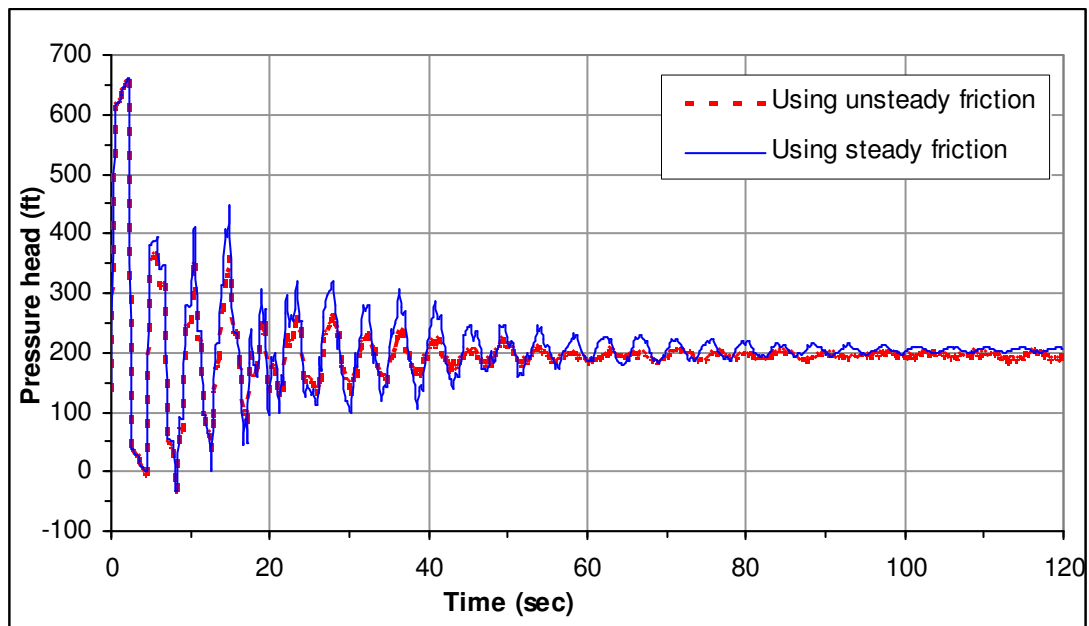
Figure 11: Effect of friction model used on transient pressure, at upstream of the valve.
