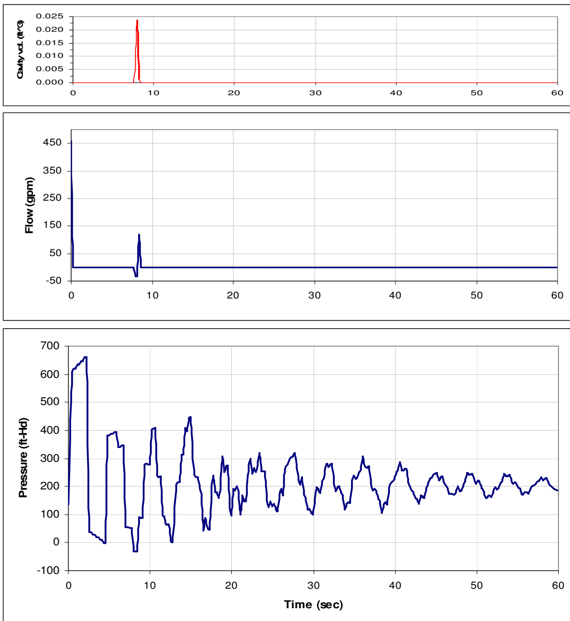
Figure 2: Transient history (Pressure, Flow & cavity volume) at the upstream end of the valve using closing rate (I).
