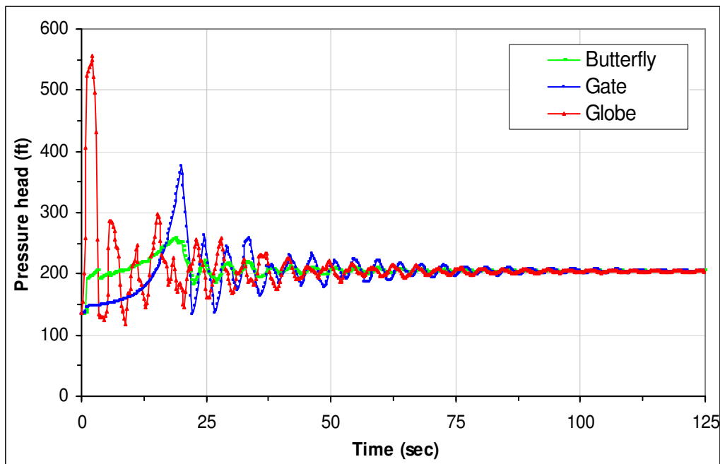
Figure 7: Effect of valve type on transient pressure head.
