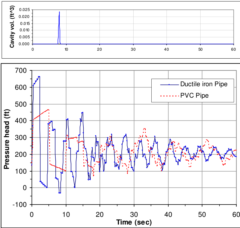
Figure 8: Effect of using PVC pipes on the local pressure head variations and cavity volume at the end of pipe 5 with closing valve rate (I).
