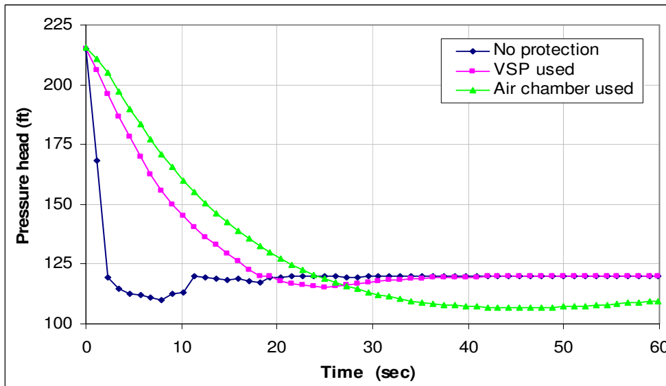
Figure 9: Effect of protection device on local transient pressure at pump discharge side
