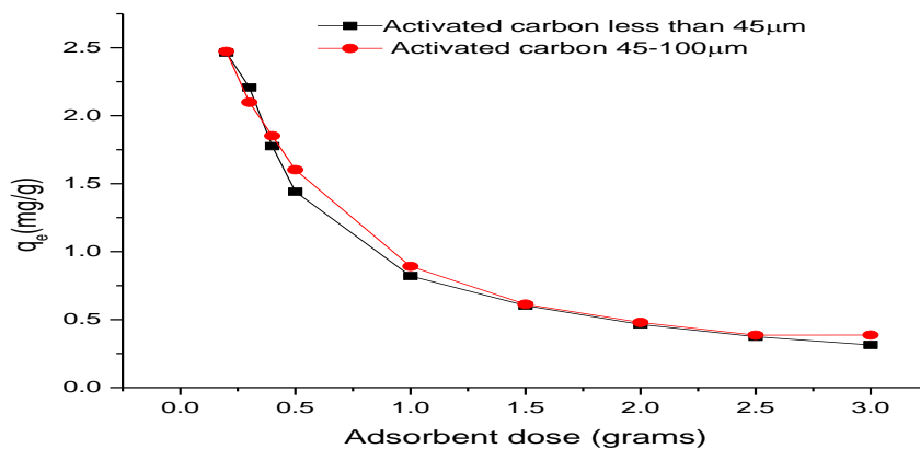
Figure3. Effect weight of adsorbent active carbon (100-45um) and (less than 45µm) on adsorption capacity, 20.08ppm dye concentration, connect time 120 min and at 25°C.
