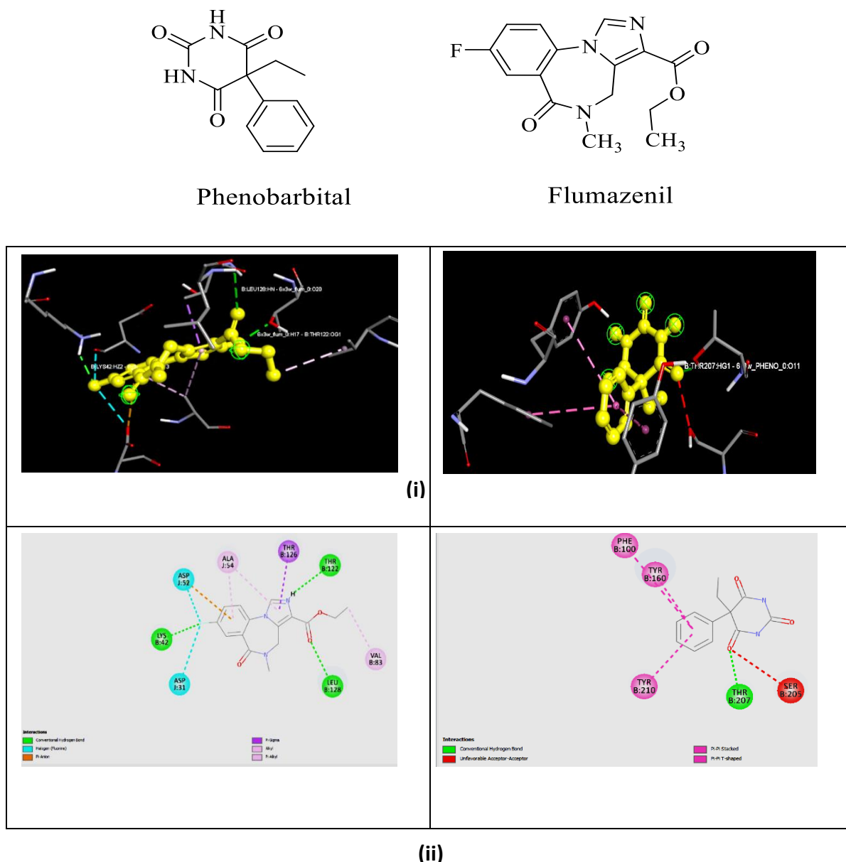
Figure 1: (i) Localization of flumazenil and phenobarbital (yellow shape) at active sites at GABA A (ii) 2D interactions of drugs with amino acid residues
