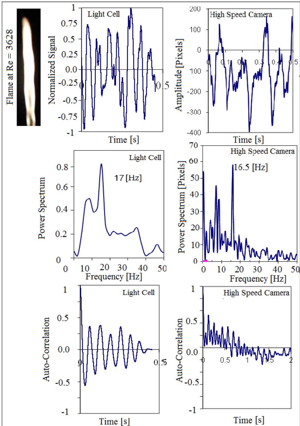
Figure 5: Flame image, Time-series, power spectrum, and auto-correlation at Reynolds number ( Re ) = 3628, by using both techniques (light cell and High speed camera)
