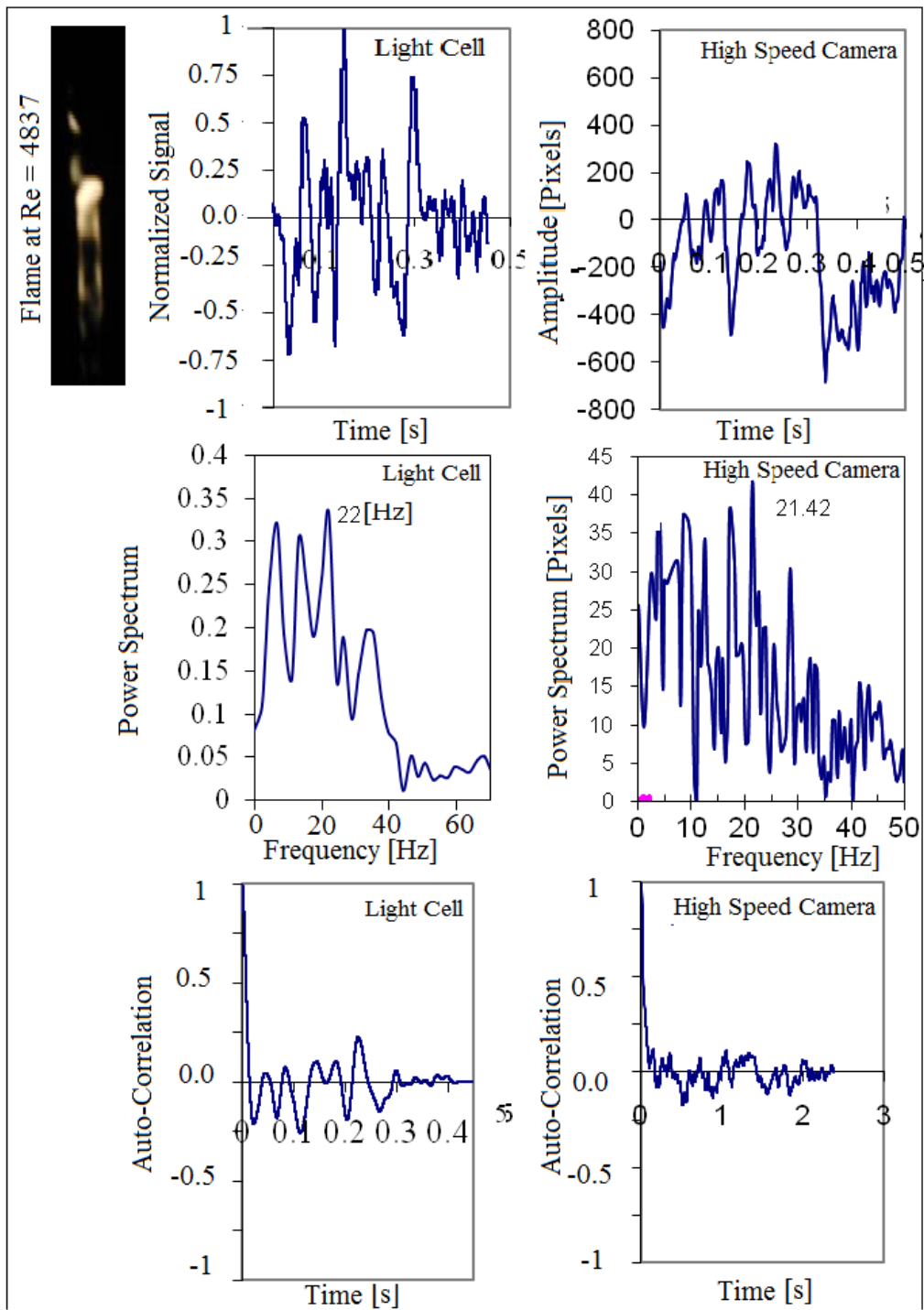
Figure 6: Flame image, Time-series, power spectrum, and auto-correlation at Reynolds number ( Re ) = 4837, by using both techniques (light cell and High speed camera)
