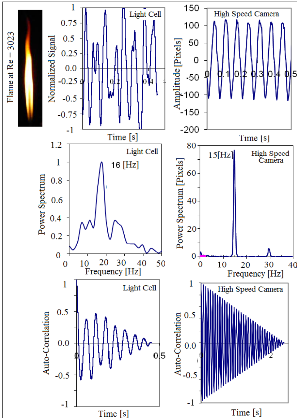
Figure 4: Flame image, Time-series, power spectrum, and auto-correlation at Reynolds number ( Re ) = 3023, by using both techniques (light cell and High speed camera)
