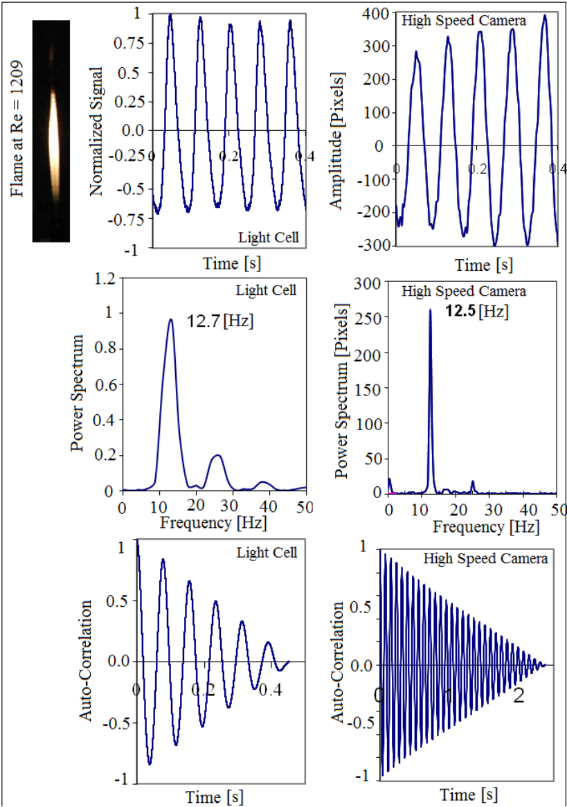
Figure 2: Flame image, Time-series, power spectrum, and auto-correlation at Reynolds number ( Re ) = 1209, by using both techniques (light cell and High speed camera)
