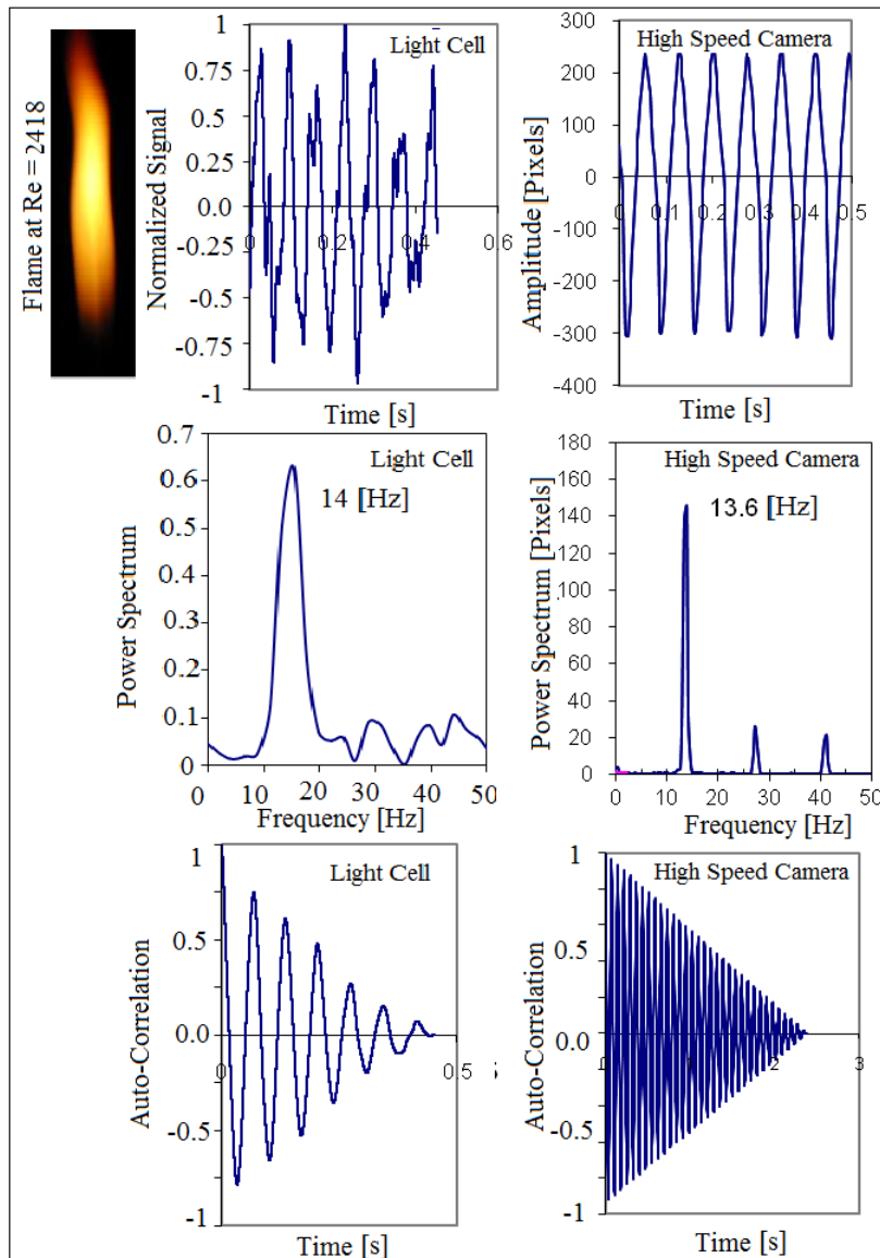
Figure 3: Flame image, Time-series, power spectrum, and auto-correlation at Reynolds number ( Re ) = 2418, by using both techniques (light cell and High speed camera)
