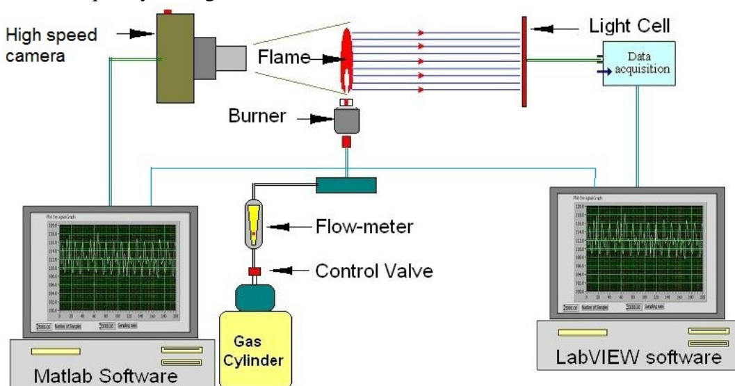
Figure 1: Schematic of the experimental configuration of the chemiluminescence measurement system.
