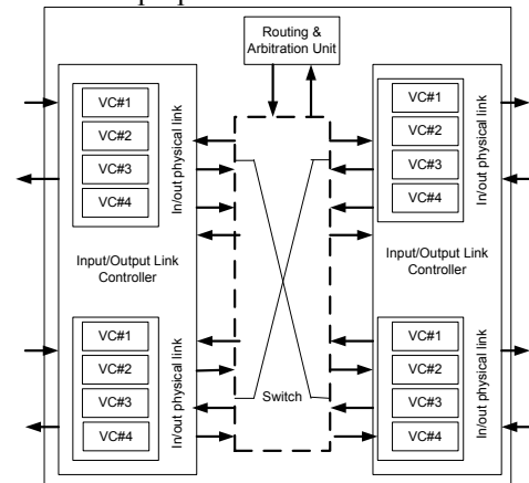
Fig.5. The top-level of the switch structure
