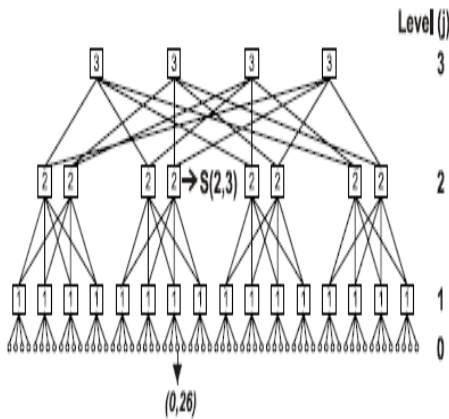
Fig.4. Butterfly fat tree structure with 64 IP cores
