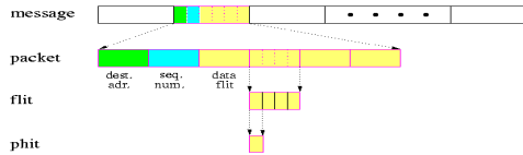
Fig. 2. Message structure (packet, flit, phit)
