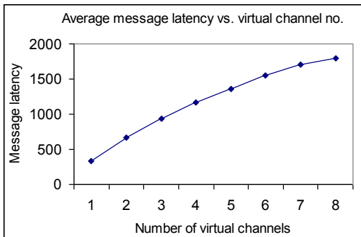
Fig.11. Average message latency vs. virtual channels
