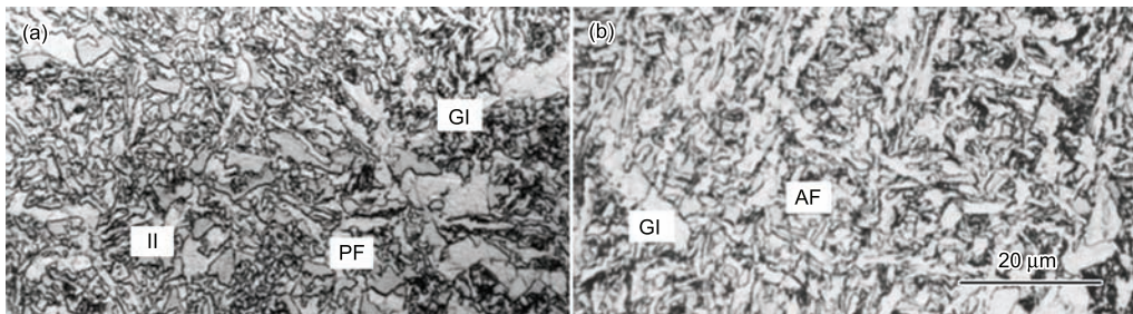
Fig. 3 Microstructure of Cr steel air-cooled from austenitization temperature of: (a) 1050 °C, (b) 1300 °C (GI–grain boundary idiormorphs; II–intragranular idiormorphs, PF–polygonal ferrite, AF–acicular ferrite)
