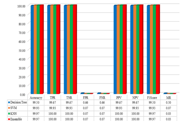
Figure 4. Simulation result based on the GoogLeNet with ACO-PSO
