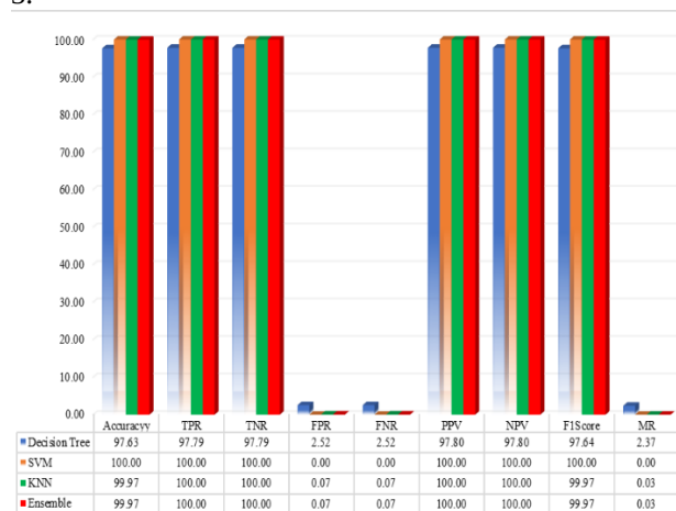
Figure 3. The result of the simulation based on the ResNet-50 and ACO-PSO
