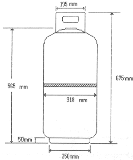
Fig.1 The LPG gas cylinder and its design parameters.
