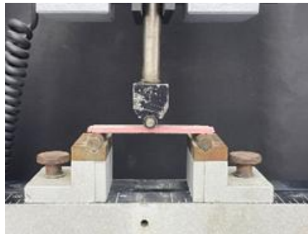
Figure 2. A sample on universal testing machine table.
