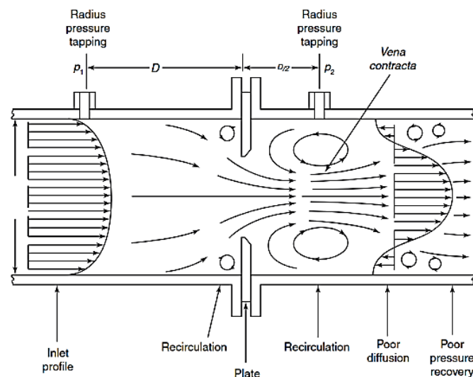
Figure 1: Geometry and flow patterns around the orifice plate flowmeter [1]
