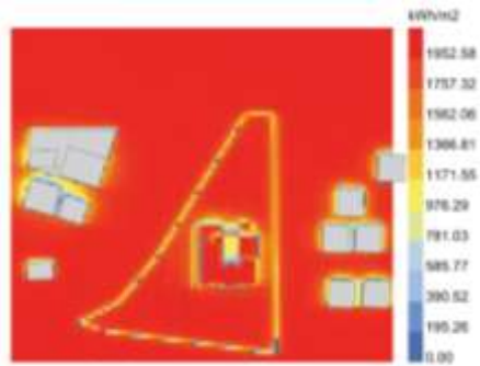
Figure 42: Incident Radiation Results – Base Model
