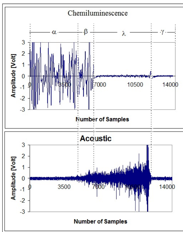
Figure 8: Time history of Chemiluminescence emission and acoustic pressure signals at H/D=1 , Burner diameter 1.2mm.
