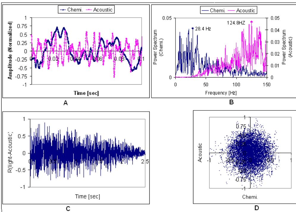
Figure 12: Time series (A), power spectrum (B), ( R_{\text{chemil.} - \text{acoustic}} ) (C), and phase space diagram (D), ( d_2=1.2\text{mm} and H/D=0.5 ).
