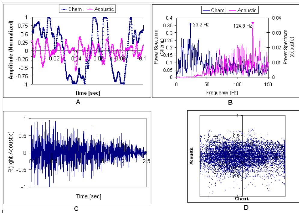
Figure 11: Time series (A), power spectrum (B), ( R_{\text{chemil.} - \text{acoustic}} ) (C), and phase space diagram (D), ( d_1=0.7\text{mm} and H/D=1 ).
