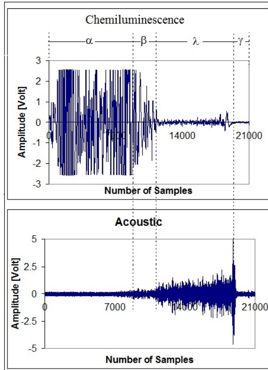
Figure 9: Time history of Chemiluminescence emission and acoustic pressure signals at H/D=1 , Burner diameter 1.7mm.
