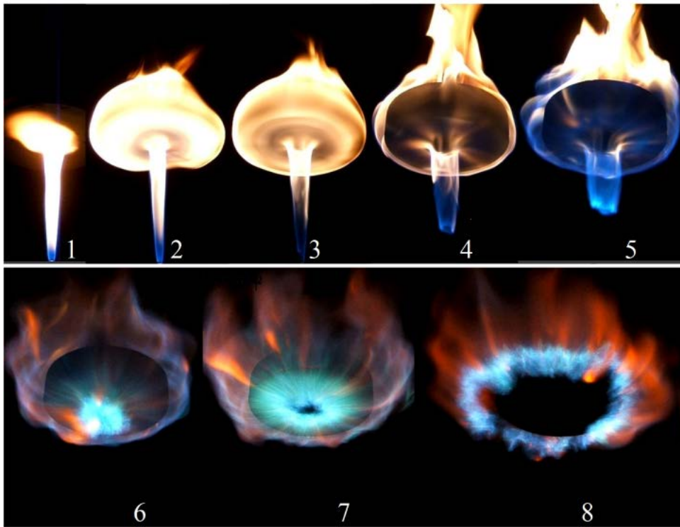
Figure 5: flame photography images during the increase of fuel flow rate from a laminar to the flame blowout conditions at H/D=1 , and Burner diameter 1.2mm.
