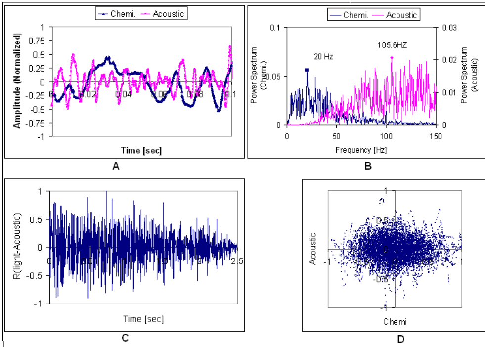
Figure15: Time series (A), power spectrum (B), ( R_{\text{chemil.} - \text{acoustic}} ) (C), and phase space diagram (D), ( d_2=1.7\text{mm} and H/D=1 ).
