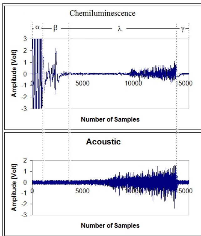
Figure 7: Time history of Chemiluminescence emission and acoustic pressure signals at H/D=1 , Burner diameter 0.7mm.
