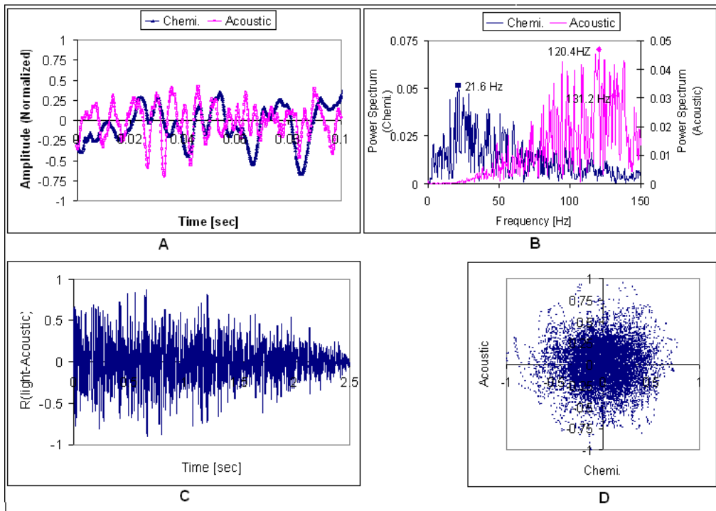
Figure 13: Time series (A), power spectrum (B), ( R_{\text{chemil.} - \text{acoustic}} ) (C), and phase space diagram (D), ( d_2=1.2\text{mm} and H/D=1 ).
