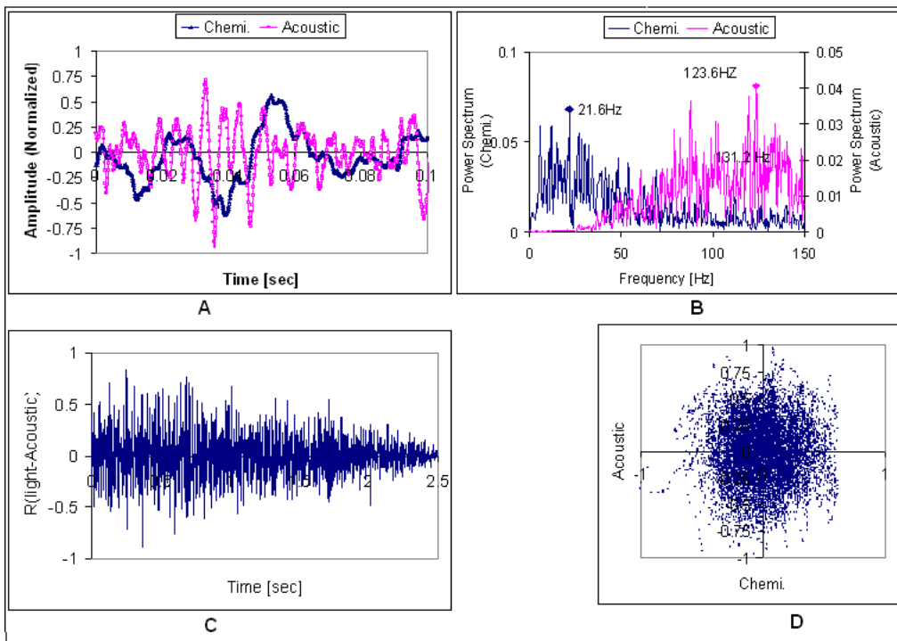
Figure 14: Time series (A), power spectrum (B), ( R_{\text{chemil.} - \text{acoustic}} ) (C), and phase space diagram (D), ( d_2=1.7\text{mm} and H/D=0.5 ).
