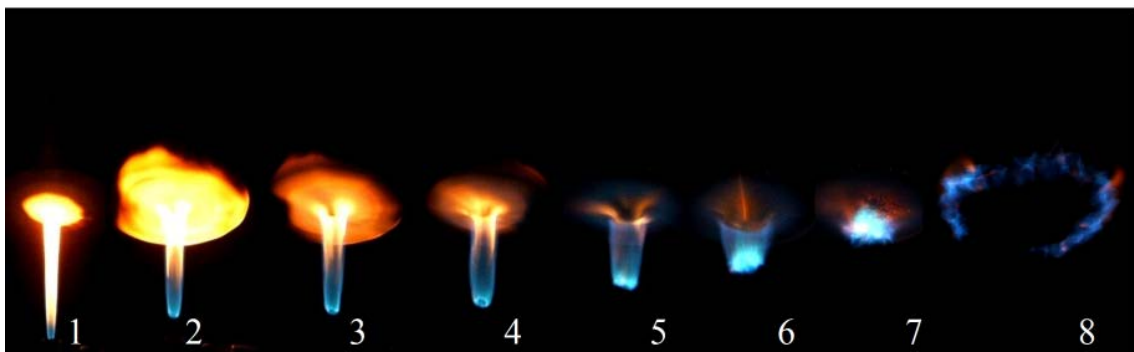
Figure 4: flame photography images during the increase of fuel flow rate from a laminar to the flame blowout conditions at H/D=1 , and Burner diameter 0.7mm
