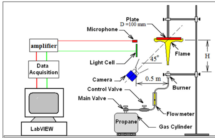
Figure 1: Layout of the Experiment.
