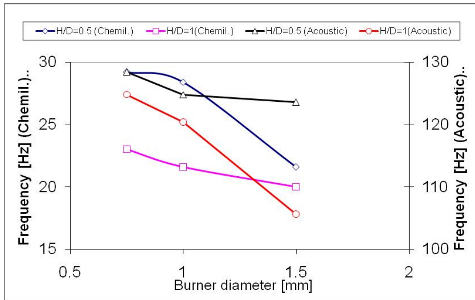
Figure 16: Burner diameter versus frequency mode of Chemiluminescence and acoustic emissions at H/D = 0.5 and 1 .
