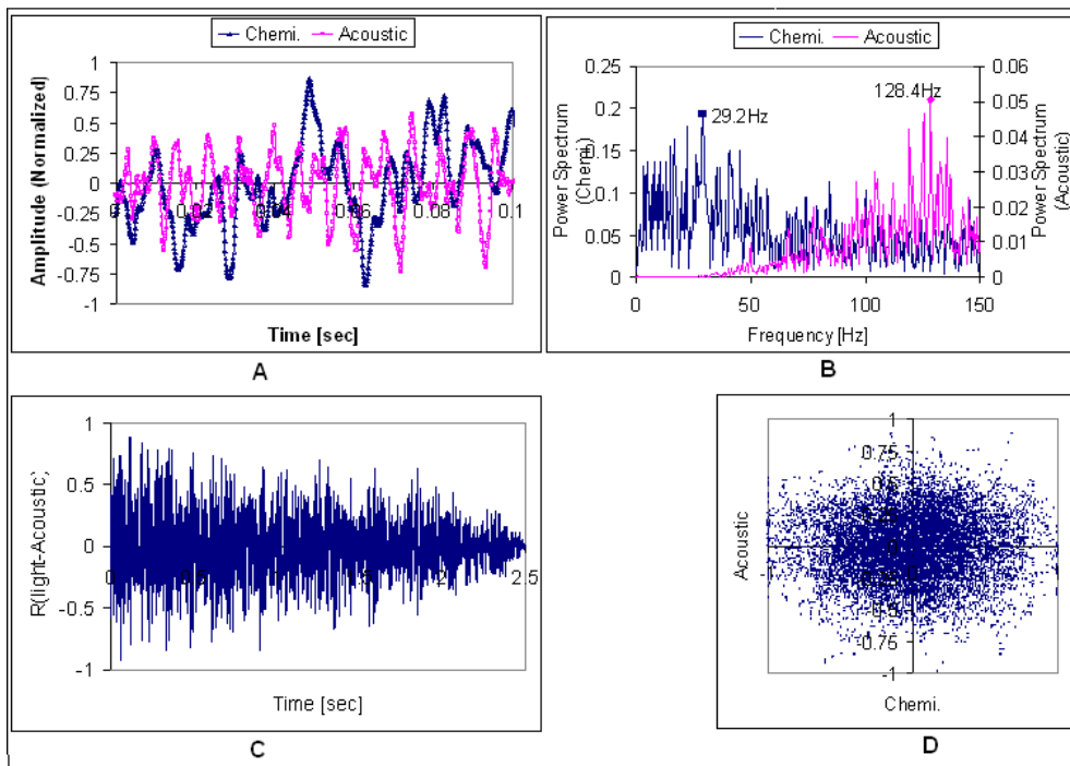
Figure 10: Time series (A), power spectrum (B), cross-correlation of ( R_{\text{chemil.} - \text{acoustic}} ) (C), and phase space diagram (D) ( d_1=0.7\text{mm} and H/D=0.5 ).
