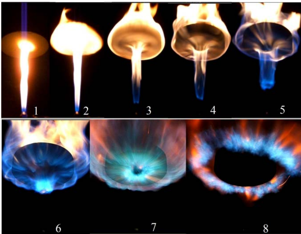
Figure 6: flame photography images during the increase of fuel flow rate from a laminar to the flame blowout conditions at H/D=1 , and Burner diameter 1.7mm.
