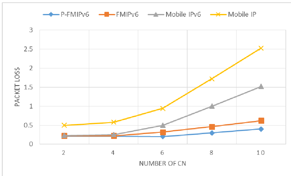
FIGURE 4: Impact of Packet Loss.
