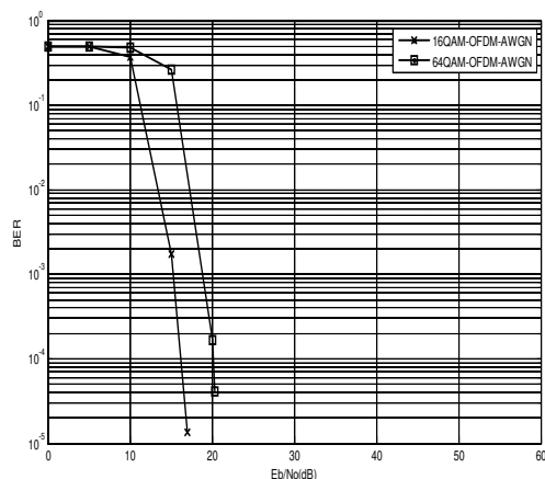
Figure 6: BER vs E_b/N_0 plots for [16QAM-OFDM & 64QAM-OFDM] AWGN channel using channel coding .
