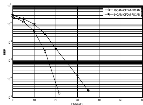
Figure 4: BER vs E_b/N_0 plots for 16QAM-FDM & 64QAM-OFDM] Rician channel
