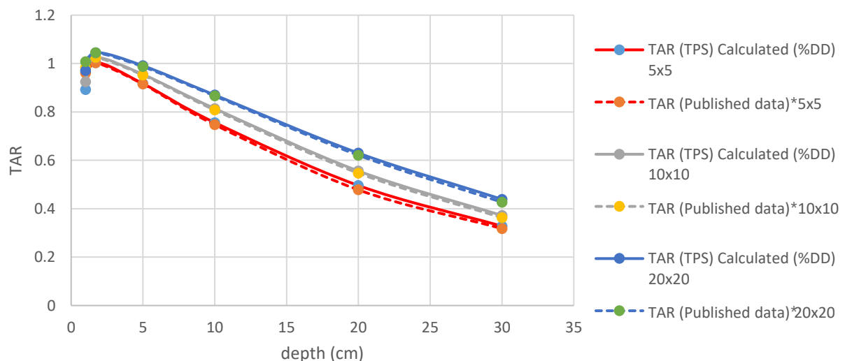
Figure (6): the comparison between the calculated Tissue Air Ratio (TAR) values derived from Treatment Planning System (TPS) calculations (based on %DD) with published reference data for various field sizes (5×5, 10×10, and 20×20 cm²) .
