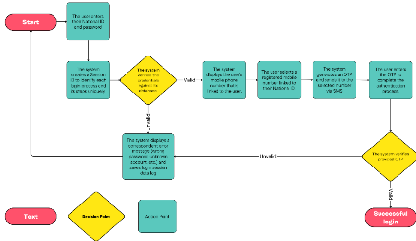
Fig. 1. The authentication process flow
