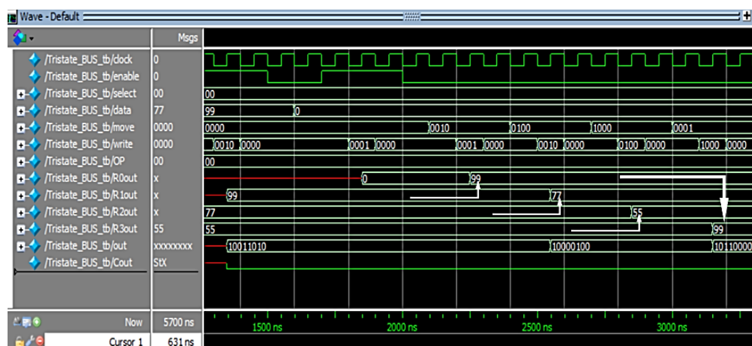
Figure 5. the transfer via bus to different registers.
