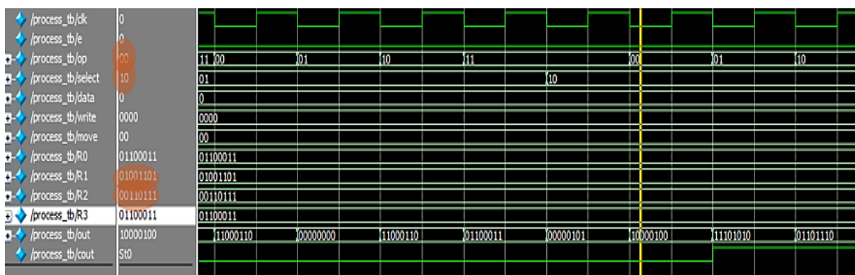
Figuer 9. ALU "ADD" operation.
