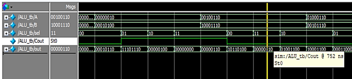
Figure 3. ALU operation.
