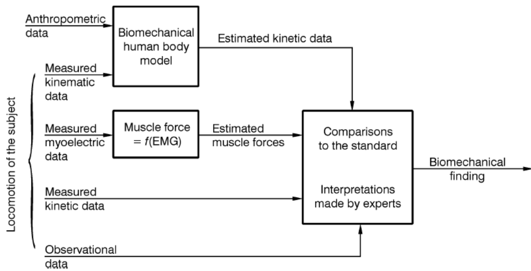
FIGURE 3.5 Information flow in a clinical locomotion measurement system.
